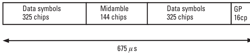
Figure 7.14 Slot structure. (© 2001 3GPP.)
