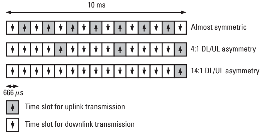
Figure 7.6 Uplink and downlink slot allocation scenarios, and slot structure. (© 2001 3GPP.)
