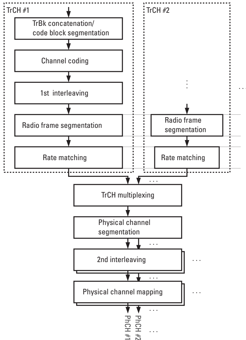
Figure 7.5 Mapping from MAC layer PDUs to physical channels. (© 2001 3GPP.)
