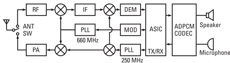
Figure 8.9 System block diagram. (Source: [6], © 1994, IEICE.)
