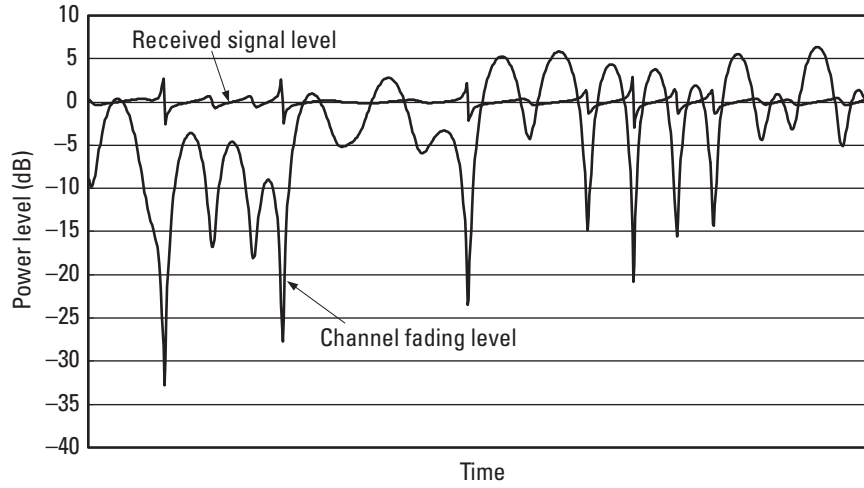
Figure 4.10 Power control error due to channel estimation error.
