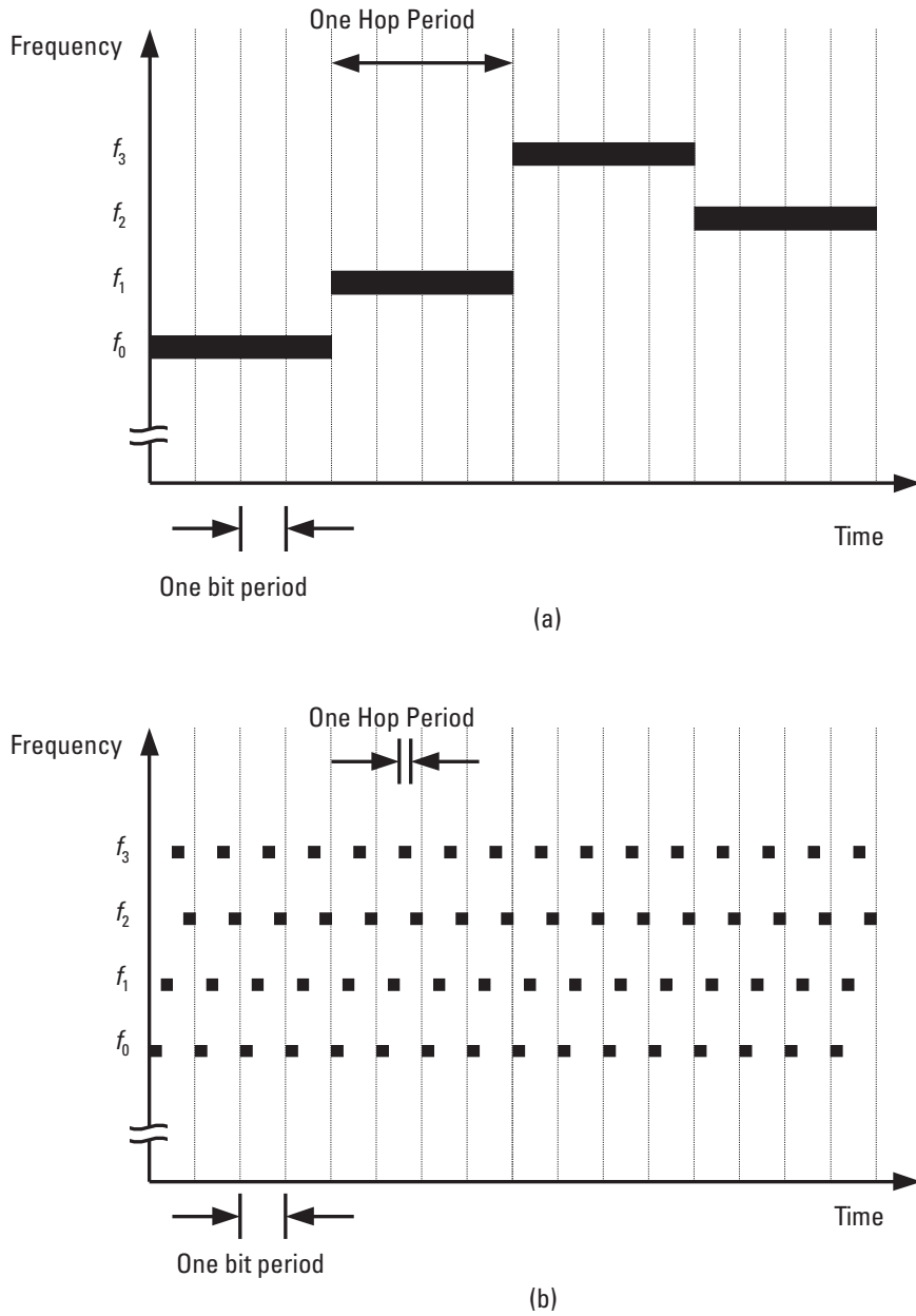
Figure 2.16 A frequency versus time diagram of the two different types of FH-SS systems: (a) SFH-SS and (b) FFH-SS.
