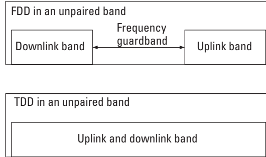
Figure 3.8 Uplink and downlink channel assignment in TDD and FDD modes of an ISM band operation.
