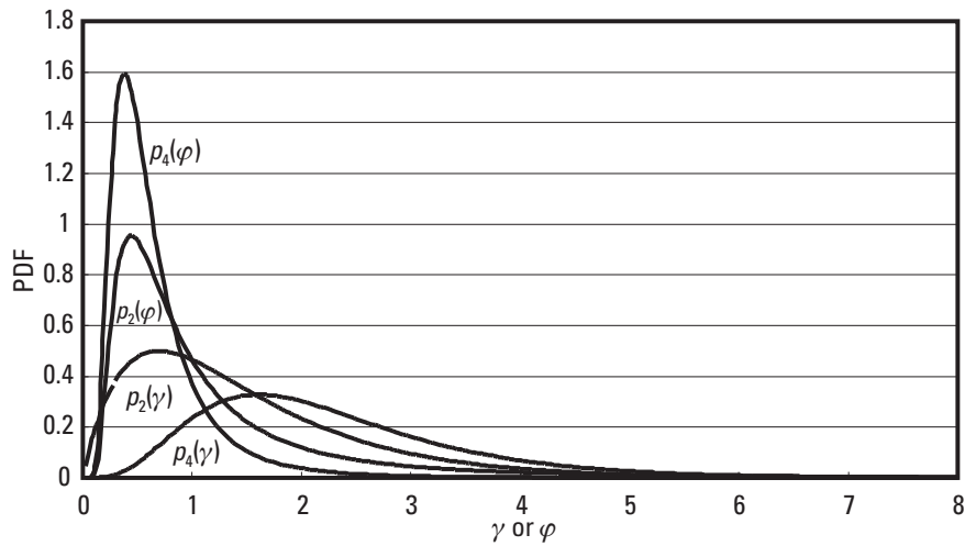
Figure 4.14 PDF for \gamma and \varphi for selection diversity systems of two and four paths.
