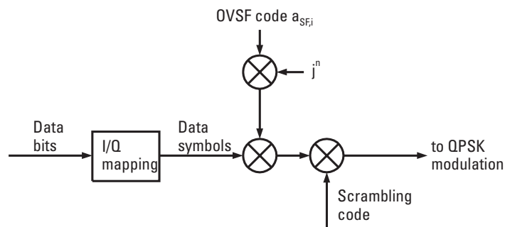
Figure 7.8 Modulation. (© 2001 3GPP.)
