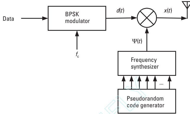
Figure 2.14 Block diagram of an FH-SS transmitter.
