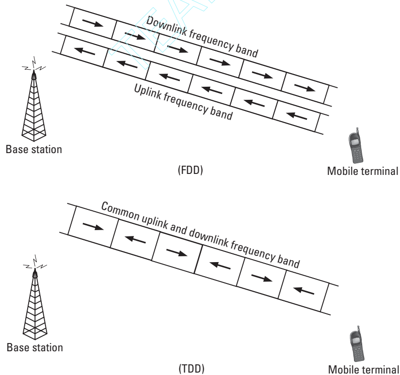
Figure 1.4 TDD and FDD.
