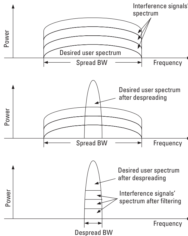
Figure 2.21 Signal and interference power before and after despreading.
