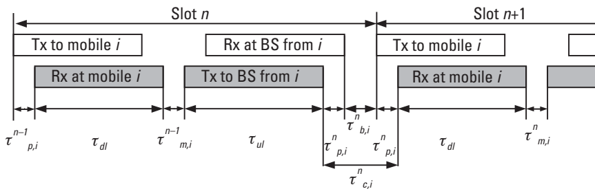
Figure 6.6 The control clock \tau_{c,i}^n .
