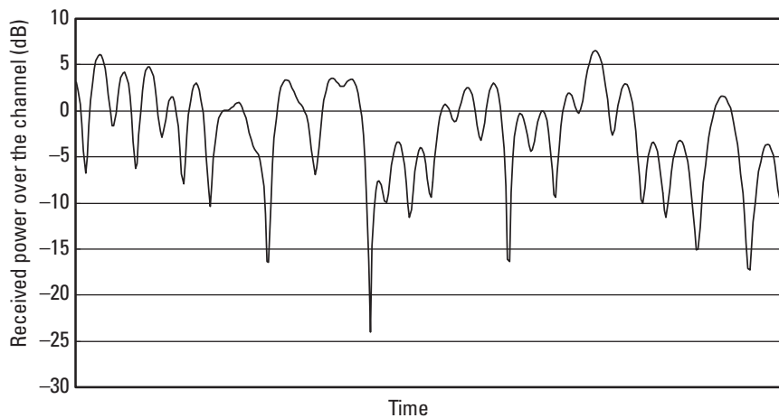
Figure 2.7 The variation of a received signal level over time as a result of the fading process.
