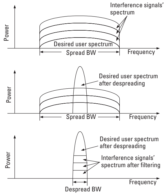
Figure 6.1 Multiuser interference, SIR.
