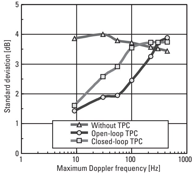
Figure 7.16 TPC error. (Source: [15], © 1998 IEICE.)
